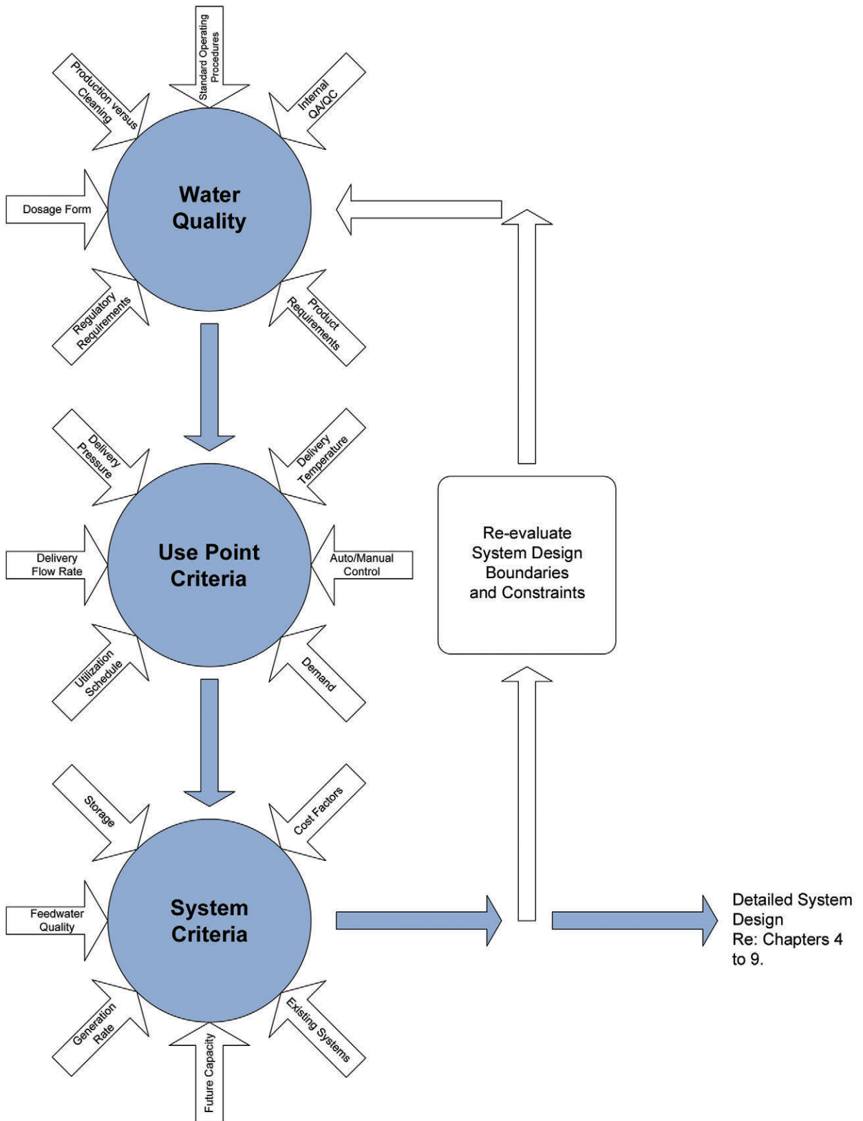
Figure 3.2: Pharmaceutical Water System Planning
