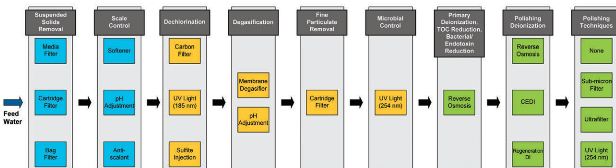
Figure 6.5: Membrane-Based Water for Injection System Technology Map
