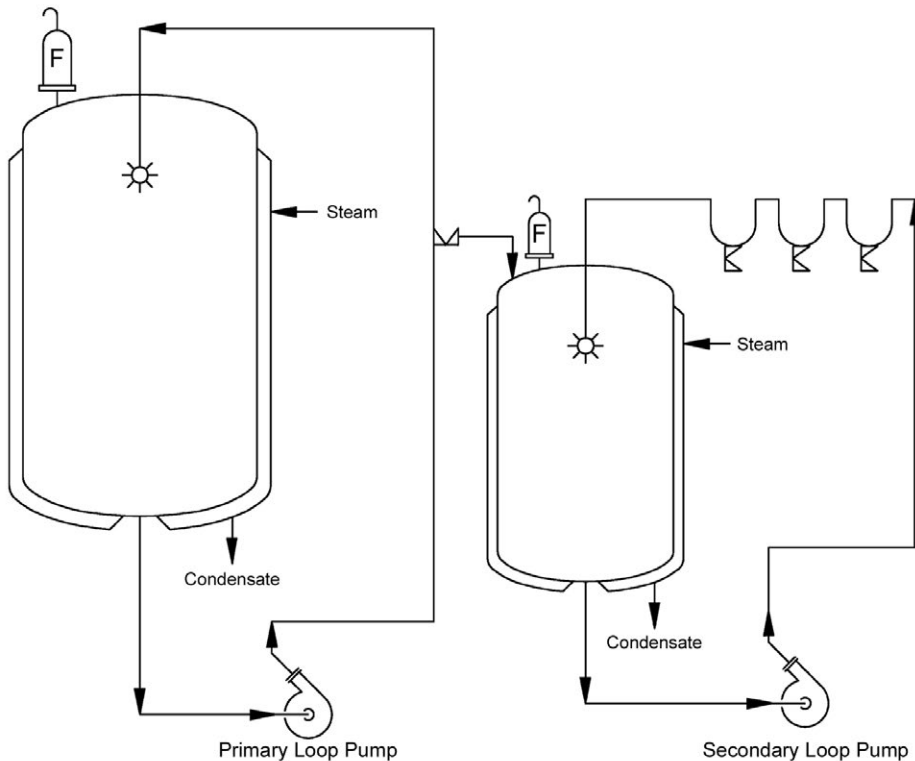
Figure 8.12: Primary/Secondary Distribution
